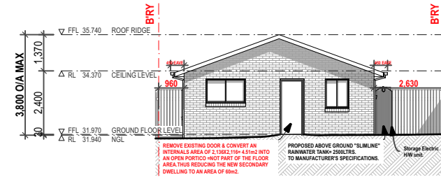
FRONT ELEVATION-WEST 1:200
