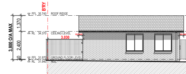
SIDE ELEVATION-NORTH 1:200
