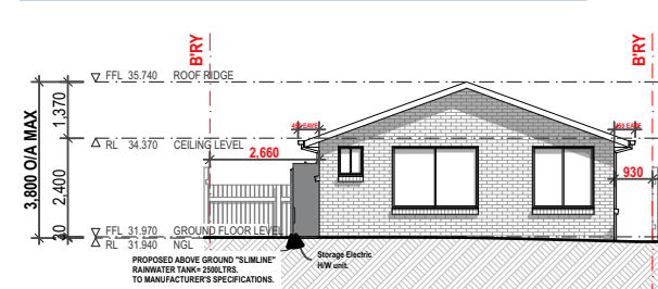
REAR ELEVATION-EAST 1:200
