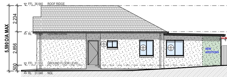
SIDE ELEVATION-SOUTH 1:200
