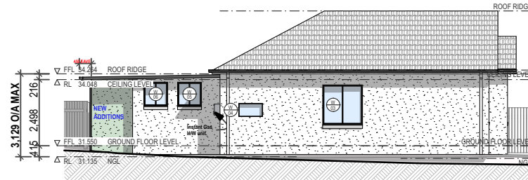
SIDE ELEVATION-NORTH 1:200
