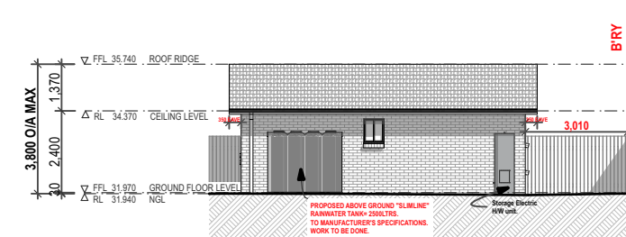
SIDE ELEVATION-SOUTH 1:200
